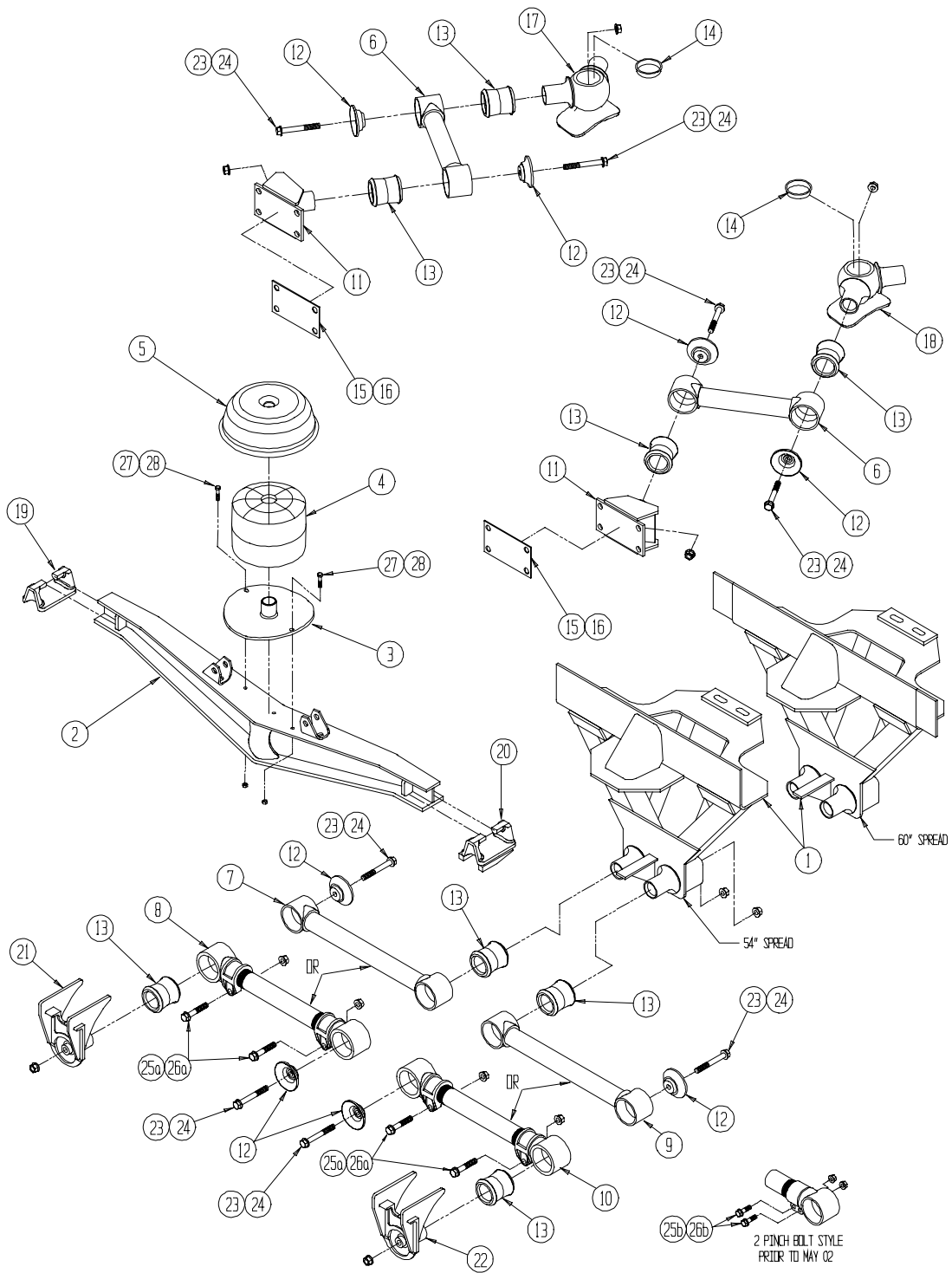
Chalmers Suspensions 800 Series 40,000 lbs. Tandem Truck Suspension
